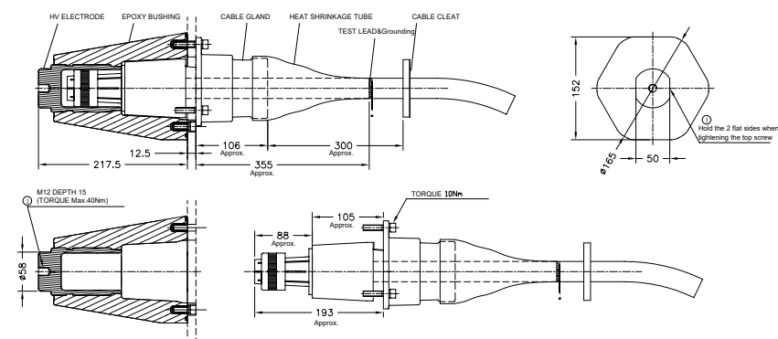
RPIT Inner Cone Size 3XL 800-1000 mm²
